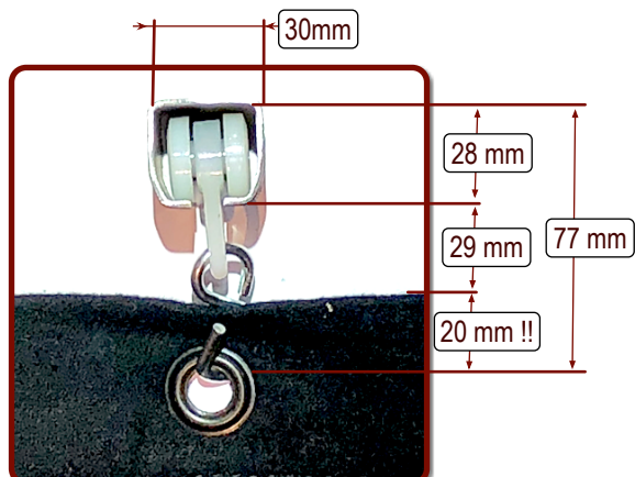
Art.Nr.: 7007bs in Track-100 Schiene
